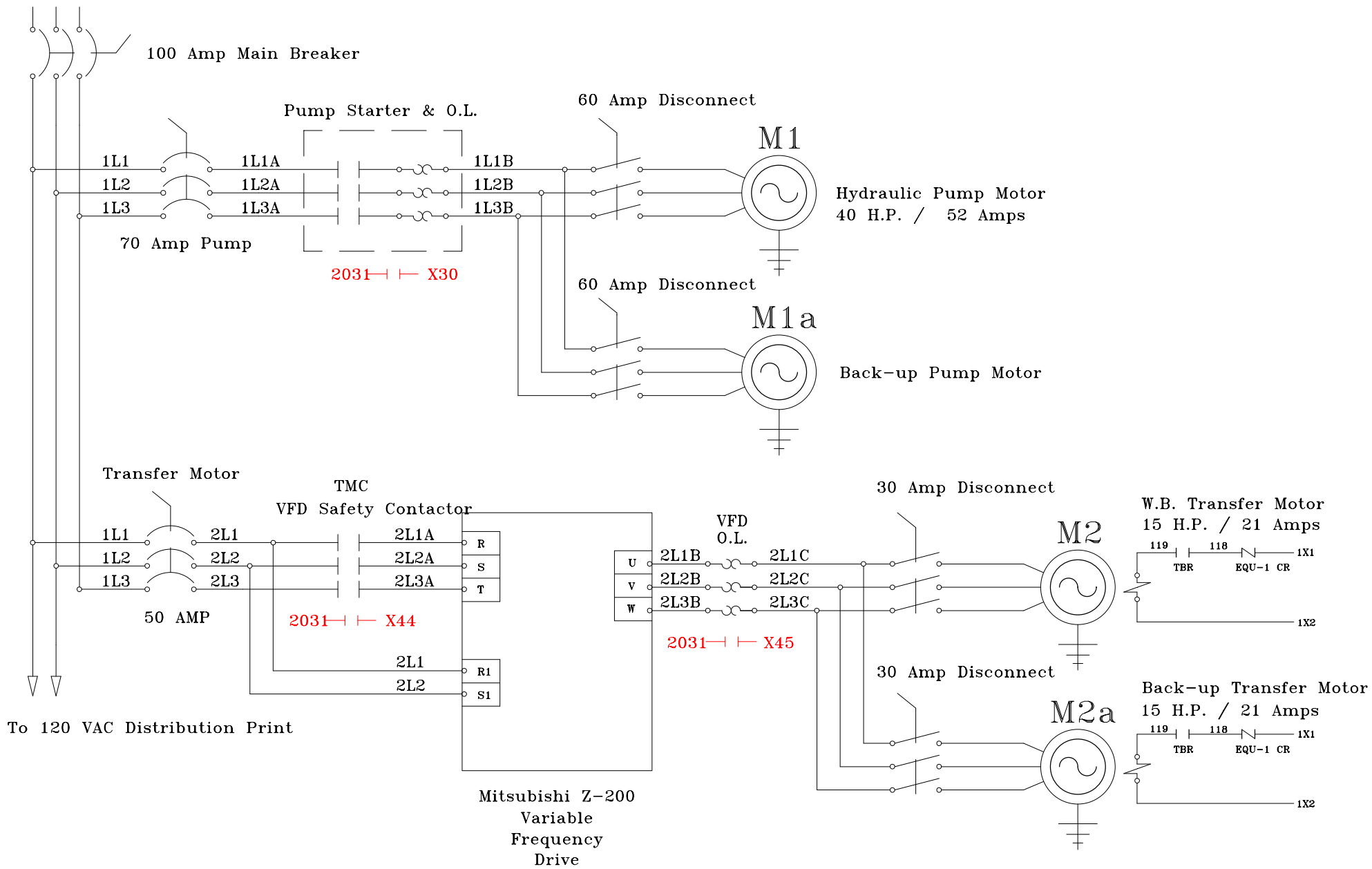
Walking Beam 3 Phase 480 VAC Distribution
